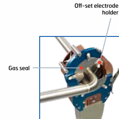
Elbow kit
